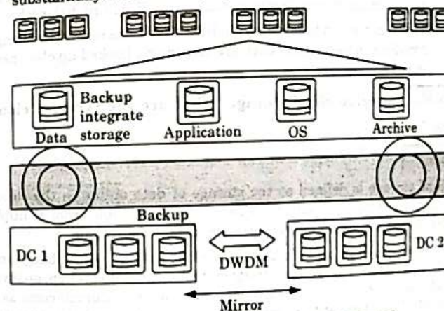
Fig. 3.29.1. Storage resource : backup-integrated, read-only and archive storage.
