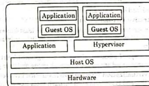
Fig. 2.25.2. OS virtualization.
