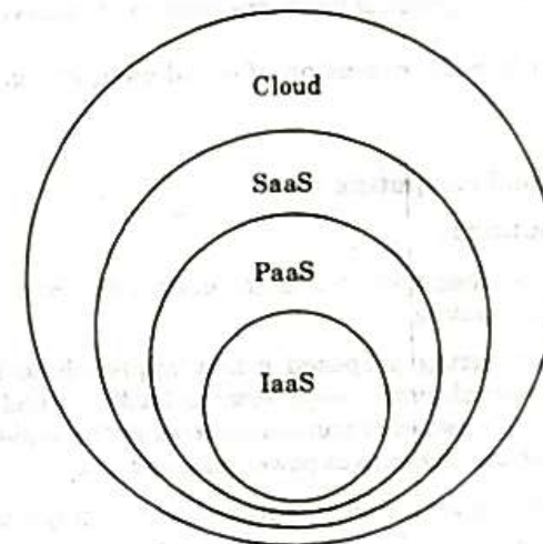
Fig. 1.11.1. Cloud services.
